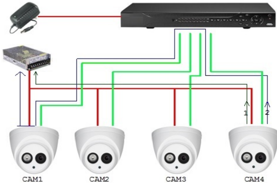
Figure 12-1 Principle of centralized power supply
