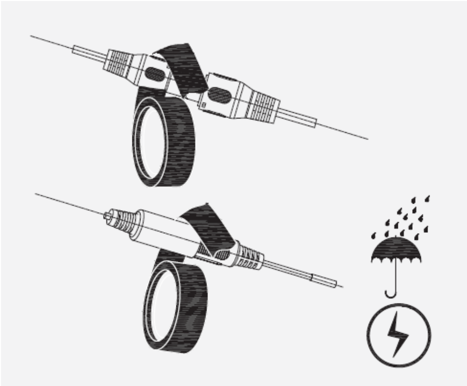
Figure 12-2 Waterproof measures
